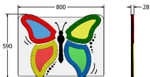
FIBUTTERFLY6
