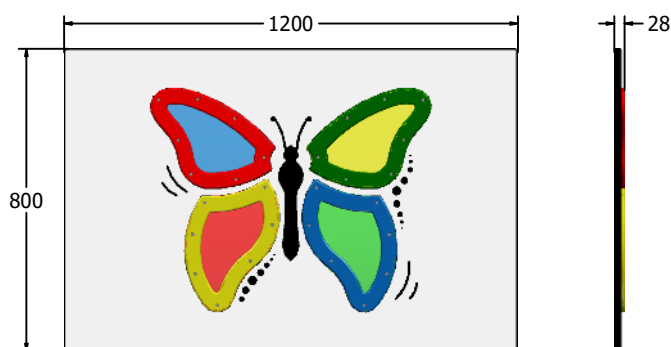
FIBUTTERFLY3
