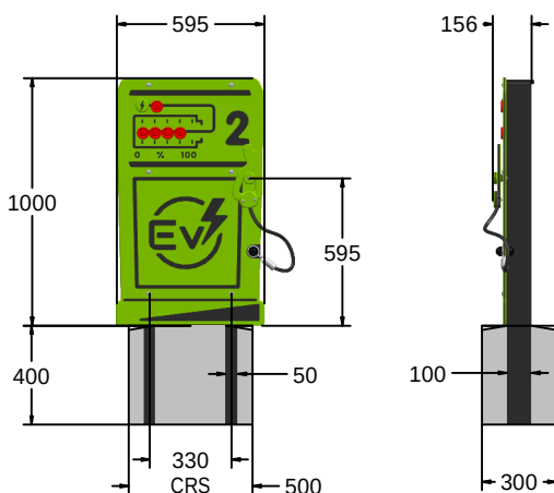
FIEVCHAR-WP - EV Charge Station Play Panel - With Posts
