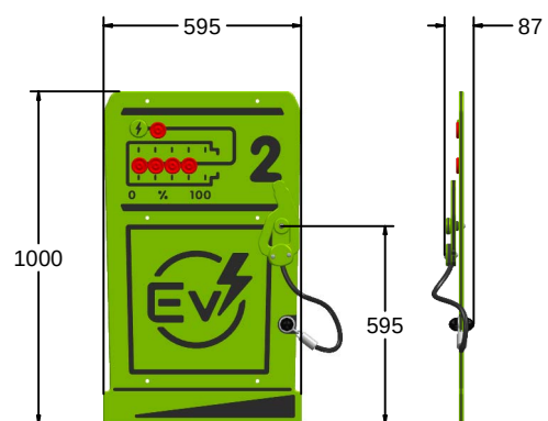
FIEVCHAR - EV Charge Station Play Panel
